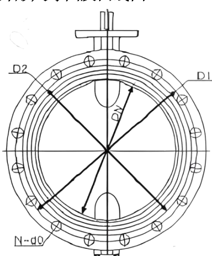
KD41/341X-10 KD41/341X-16 结构图
